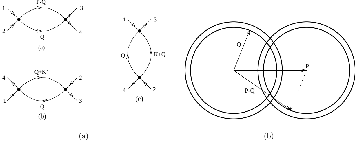
Figure 6: (a) second order diagrams renormalizing the coupling function. Here \mathbf{P} = \mathbf{K}_1 + \mathbf{K}_2 , \mathbf{K}_3 = \mathbf{K}_1 - \mathbf{K} , and \mathbf{K}_4 = \mathbf{K}_1 - \mathbf{K}' . \mathbf{Q} is the loop integration variable. Note that these diagrams are actually identical to those occurring in Landau's theory (fig.3b). (b) phase space for diagram (a). The rings are the degrees of freedom to be integrated out between \Lambda and \Lambda/s . Note that only if \mathbf{P} = 0 are \mathbf{Q} and \mathbf{P} - \mathbf{Q} simultaneously in the area to be integrated, giving a contribution of order d\ell .
