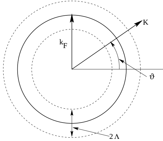
Figure 5: Fermi surface geometry in two dimensions.
