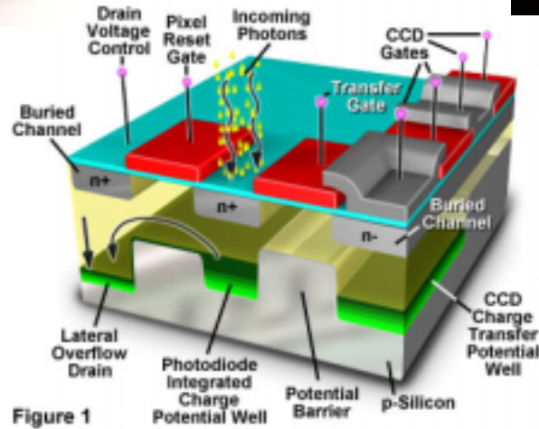
Anatomy of a Charge Coupled Device (CCD)
