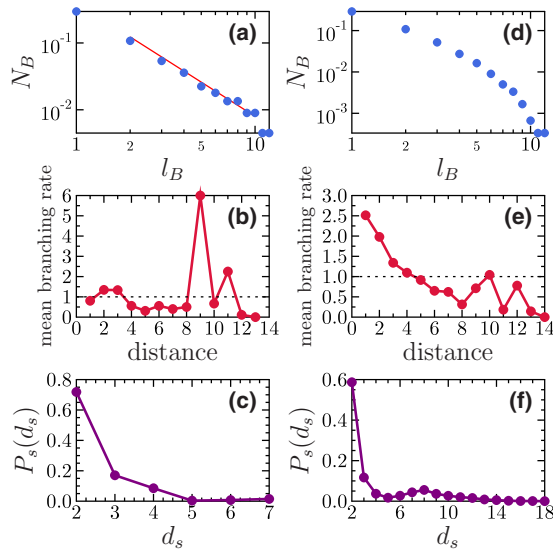
FIG. 3. (Color online) Fractal analysis of the giant component. (a) Box-covering analysis of the giant component in February 2004. N_B(l_B) , the number of boxes needed to cover an object with box size l_B , decays algebraically in l_B as N_B(l_B) \sim l_B^{-d_B} with d_B \approx 1.7 , indicating that the network is a fractal. The guideline has a slope of -1.7 , drawn for the eye. (b) Mean branching rate as a function of distance from a root node. To measure this, one identifies the skeleton [25] of the network and its largest hub as the root node. Then we calculate the average branching number in the skeleton as a function of distance from the root. The plateau around the unity value indicates that its branching pattern is that of a critical branching tree, which is a fractal. (c) The distribution of shortcut lengths. By decomposing the network into the skeleton and the residual links, we define the distance along the skeleton between two nodes connected by each residual link as the shortcut length. The shortcut length distribution of the February 2004 network has a peak at d_s = 2 and decrease monotonically as d_s increases. In (d)–(f), we measure same quantities for the network in December 2008, finding that (d) the box number decreases exponentially with the box size, (e) the mean branching ratio does not exhibit a plateau but decreases steadily as a function of the distance from the root, and (f) the shortcut length distribution becomes bimodal with an additional peak at d_s = 8 due to the long-range links. These results indicate that the network is no longer a fractal in December 2008.
