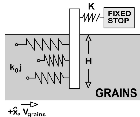
FIG. 1. Schematic illustration of the stochastic spring model. The shaded area indicates the granular medium, which moves with velocity v in the positive x direction. The motion of the cylinder that tries to move along with the grains is opposed by a fixed stop coupled to the cylinder through a spring with spring constant K . We model the grains opposing the movement as springs with spring constant k_0j .
